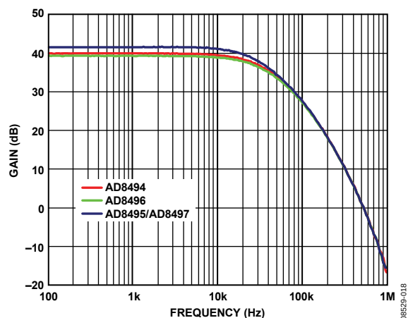
Figure 5. Frequency Response
