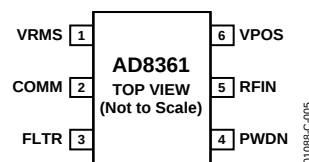
Figure 5. 6-Lead SOT-23
