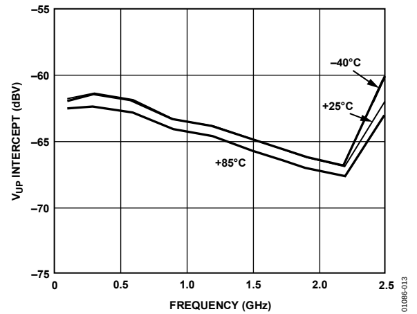
Figure 13. V_{UP} Intercept vs. Frequency; -40^{\circ}\text{C} , +25^{\circ}\text{C} , and +85^{\circ}\text{C}
