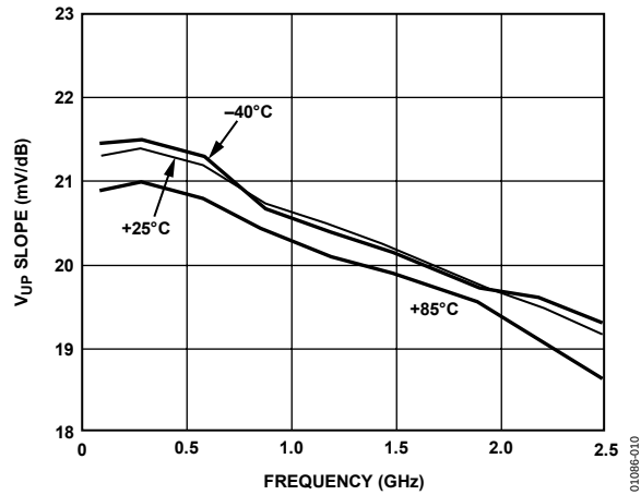
Figure 10. Slope vs. Frequency; -40^{\circ}\text{C} , +25^{\circ}\text{C} , and +85^{\circ}\text{C}
