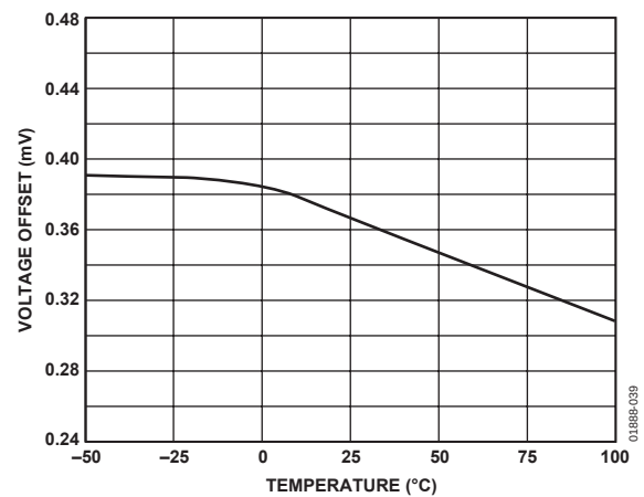
Figure 39. V_{\text{os}} vs. Temperature
