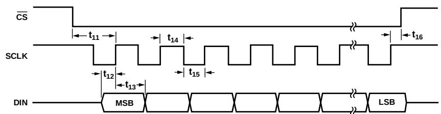
Figure 9. Write Cycle Timing Diagram
