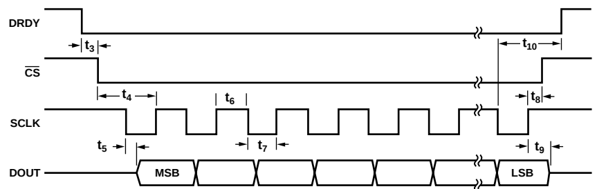
Figure 8. Read Cycle Timing Diagram
