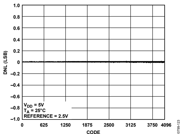
Figure 8. AD5694 DNL
