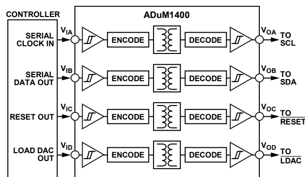
Figure 43. Isolated Interface
