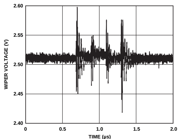
Figure 25. Digital Feedthrough
