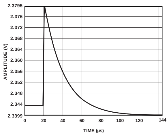
Figure 23. Midscale Glitch Energy, R_{AB} = 250\text{ k}\Omega
