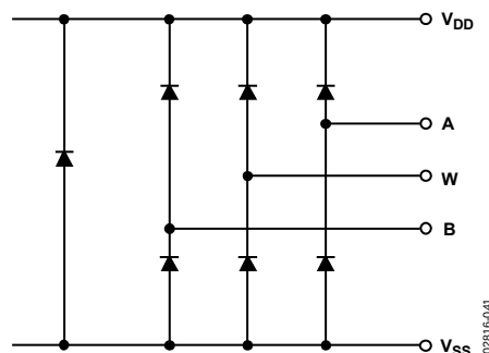
Figure 42. Maximum Terminal Voltages Set by V_{DD} and V_{SS}
