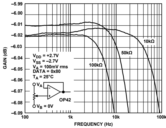
Figure 10. Gain Flatness vs. Frequency
