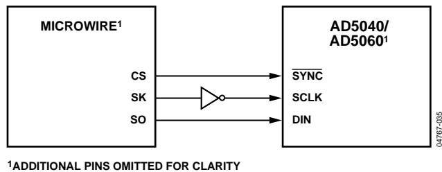
Figure 49. AD5040/AD5060 to MICROWIRE Interface
