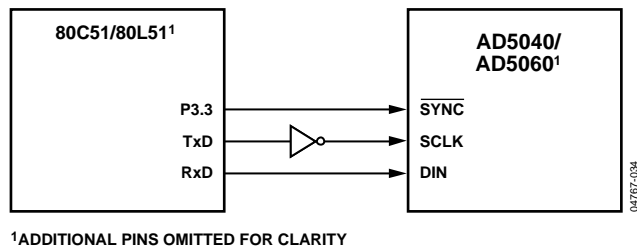
Figure 48. AD5040/AD5060 to 80C51/80L51 Interface
