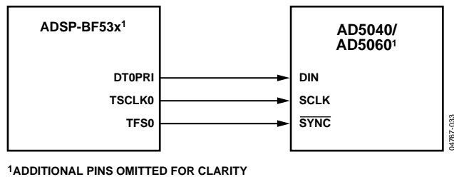
Figure 47. AD5040/AD5060 to Blackfin® ADSP-BF53x Interface
