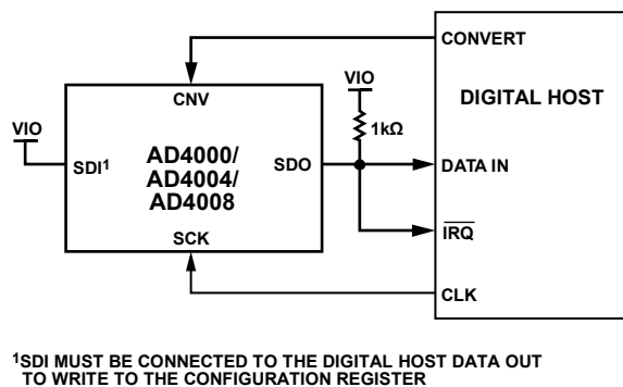
Figure 54. CS Mode, 3-Wire with Busy Indicator Connection Diagram
