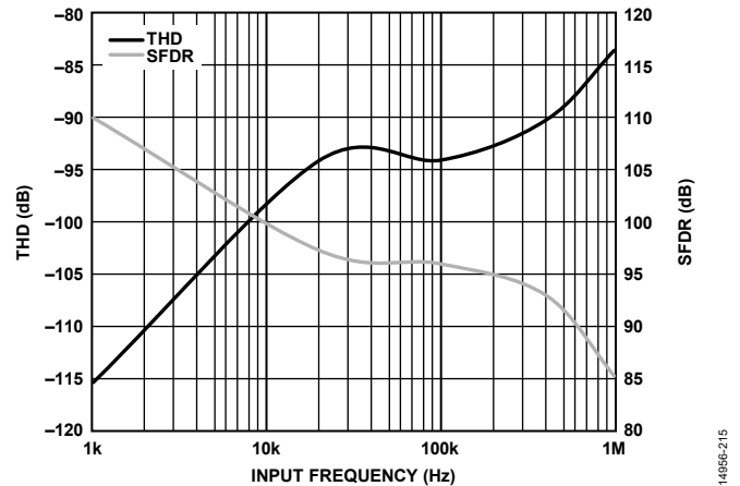
Figure 20. THD and SFDR vs. Input Frequency
