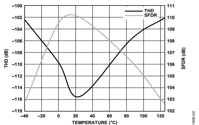
Figure 22. THD and SFDR vs. Temperature, f_{IN} = 1 kHz
