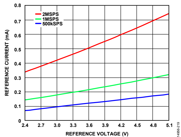
Figure 33. Reference Current vs. Reference Voltage
