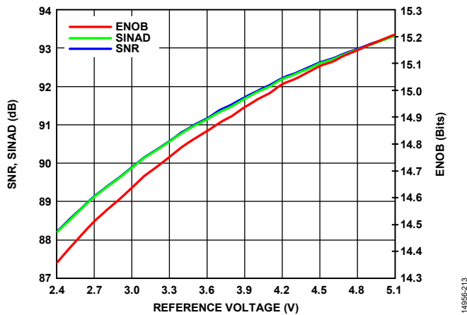
Figure 18. SNR, SINAD, and ENOB vs. Reference Voltage, f_{IN} = 1 kHz
