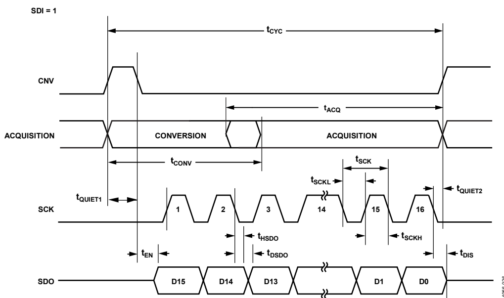
Figure 51. CS Mode, 3-Wire Turbo Mode Serial Interface Timing Diagram (Status Bits Not Shown)
