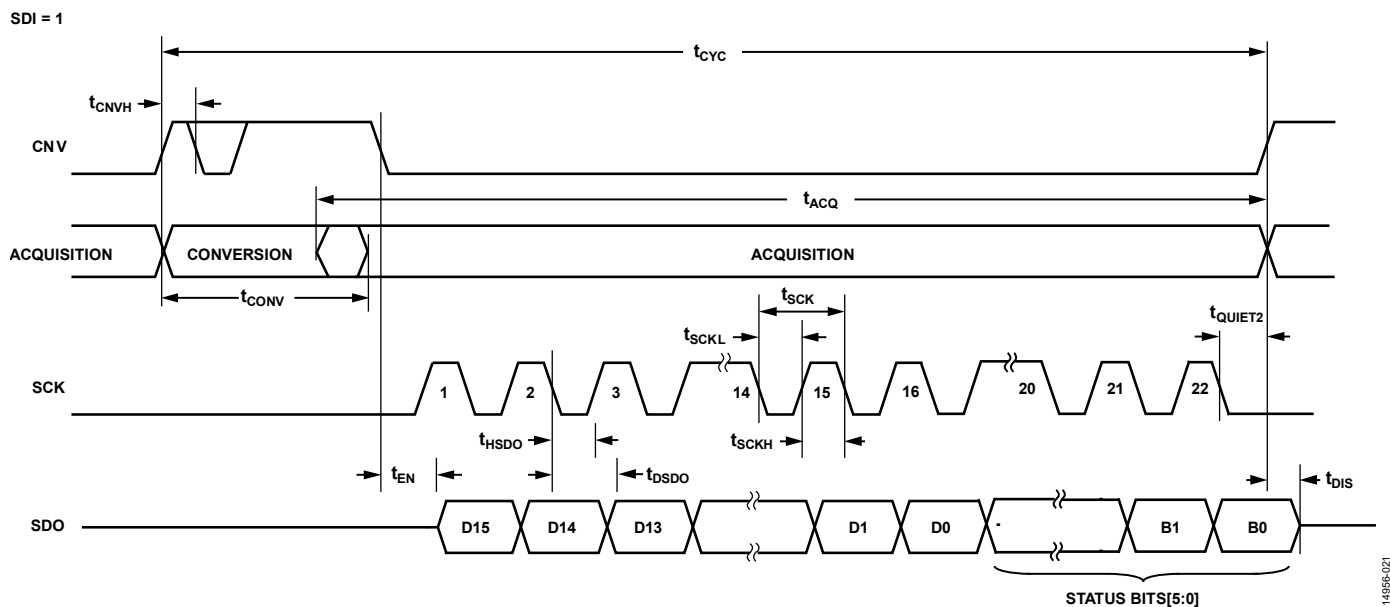
Figure 49. \overline{\text{CS}} Mode, 3-Wire Without Busy Indicator Serial Interface Timing Diagram, Including Status Bits
