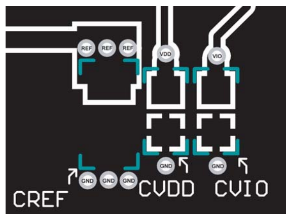
Figure 65. Example Layout of the AD4000 (Bottom Layer)
