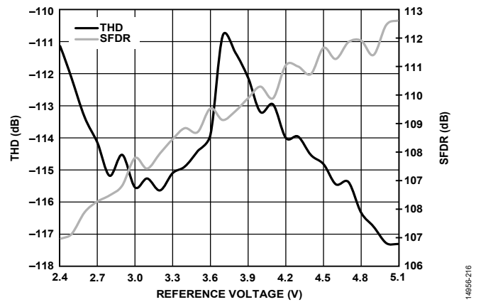
Figure 21. THD and SFDR vs. Reference Voltage, f_{IN} = 1 kHz
