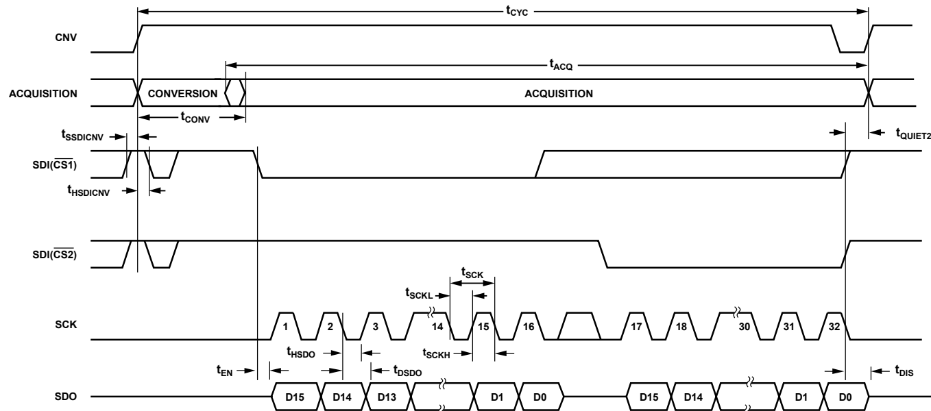
Figure 59. \overline{\text{CS}} Mode, 4-Wire Without Busy Indicator Serial Interface Timing Diagram (Status Bits Not Shown)
