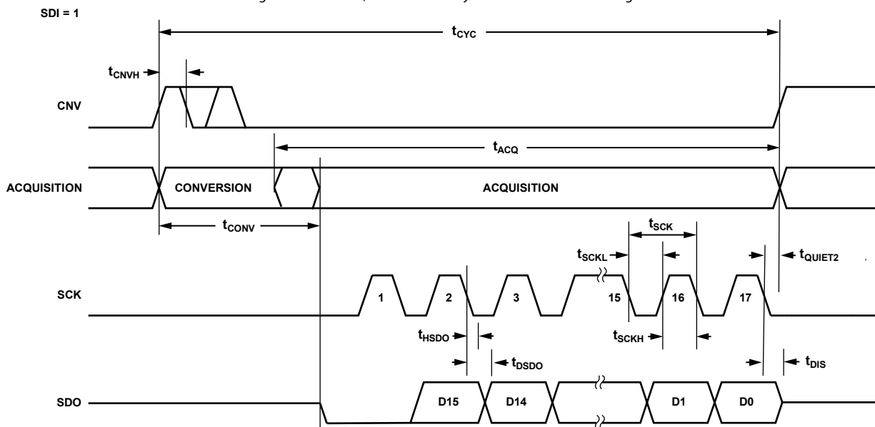
Figure 55. \overline{\text{CS}} Mode, 3-Wire with Busy Indicator Serial Interface Timing Diagram (Status Bits Not Shown)
