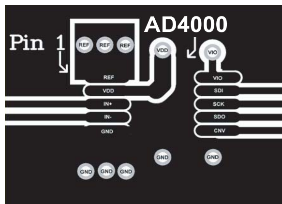
Figure 64. Example Layout of the AD4000 (Top Layer)
