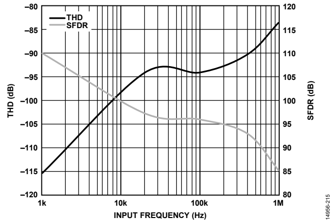
Figure 20. THD and SFDR vs. Input Frequency
