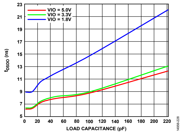
Figure 36. t_{PSDO} vs. Load Capacitance
