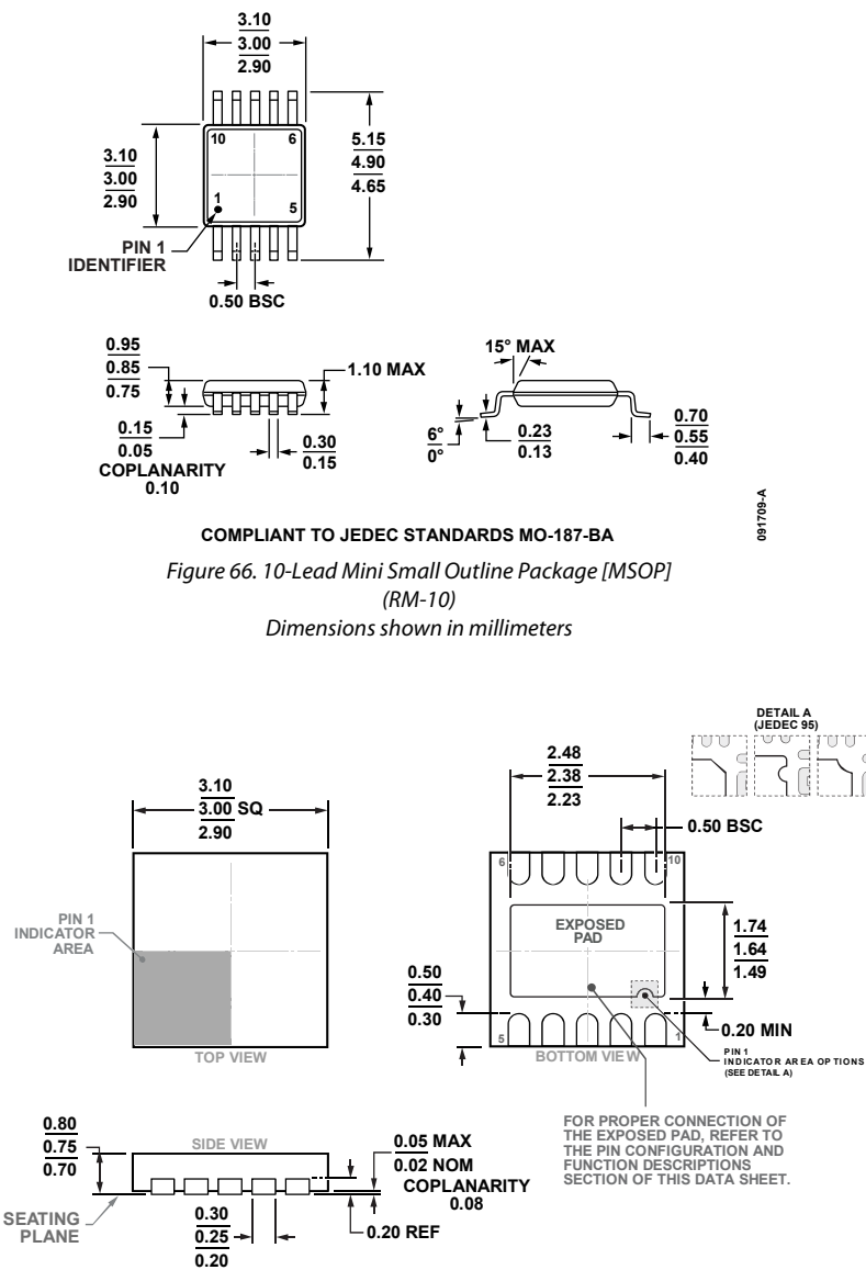
Figure 67. 10-Lead Lead Frame Chip Scale Package [LFCSP] 3 mm x 3 mm Body and 0.75 mm Package Height (CP-10-9)
