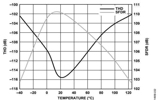
Figure 22. THD and SFDR vs. Temperature, f_{IN} = 1 kHz
