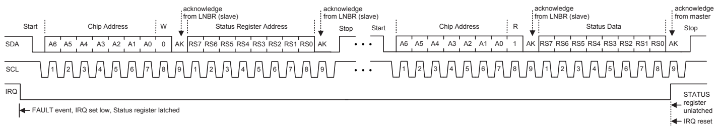
Figure 9. Fault, IRQ, and Status Register Timing. When a UVLO, OCP, or TSD event occurs, the IRQ bit is set low and the Status register is latched. The IRQ bit is reset to high when the A8298 acknowledges it is being read. The Status register is unlatched when the master acknowledges the status data from the A8298.
