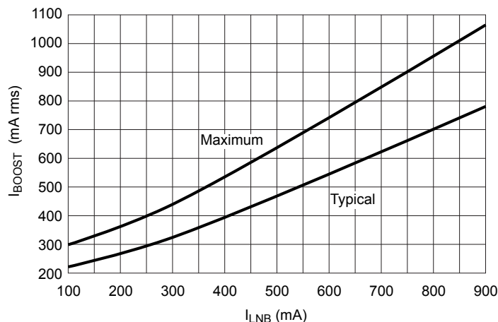
Figure 6. Boost capacitor rms current versus I_{\text{LNB}} for the A8298
