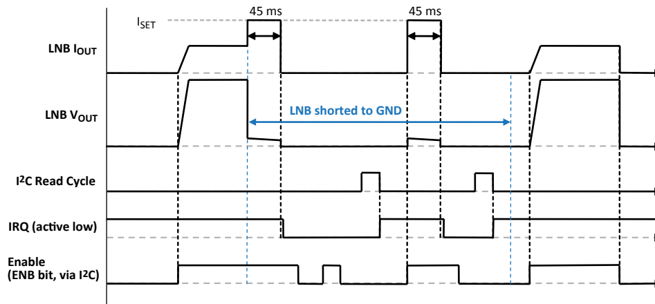
Figure 11. IRQ and Fault Clearing in Response to Overcurrent (OCP). If the LNB output is grounded for more than 45 ms, the LNB output will be shut off, an overcurrent fault (OCP) would be latched in the Status Register, and the IRQ pin would transition low. After an OCP fault, the LNB output does not respond to the Enable (ENB) bit until an I 2 C Read cycle is executed to report and clear the OCP fault. After a successful I 2 C Read, the IRQ pin transitions high and the A8298 can be re-enabled, provided the LNB output is no longer grounded.
