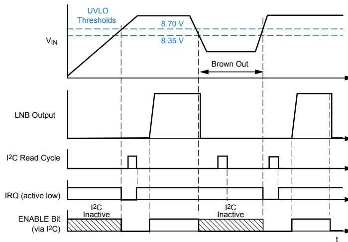
Figure 10. IRQ and Fault Clearing in Response to Undervoltage at VIN (UVLO). At power-up, while V_{IN} is below 8.70 V (typ), the A8298 is disabled and the I 2 C port is inactive. After V_{IN} rises above 8.70 V (typ), the I 2 C port becomes active and the IRQ pin is pulled low. An I 2 C Read is required to report and clear the UVLO fault and set the IRQ pin to a logic high before the A8298 can be enabled. If a brown-out occurs, such that V_{IN} drops below 8.35 V (typ), the A8298 would be disabled and the I 2 C port would become inactive (note that the IRQ pin remains high during this time because the A8298 is disabled). After V_{IN} rises above 8.70 V (typ) the I 2 C port reactivates and the IRQ pin is pulled low to report that a brown-out had occurred. An I 2 C Read is required to report and clear the UVLO fault before the A8298 can be re-enabled.
