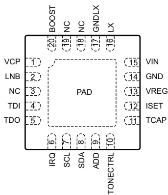
Device Pinout Diagram
