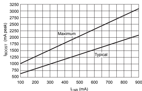
Figure 4. Boost inductor peak current versus I_{\text{LNB}} for the A8298
