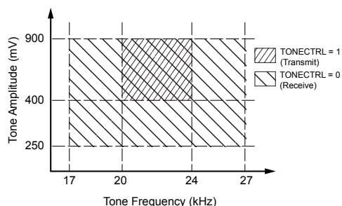
Figure 3a. Accept Ranges of Tone Detection feature
