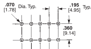
Recommended PC Board Hole Layout Mounting Dimensions
