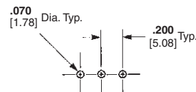
Recommended PC Board Hole Layout Mounting Dimensions
