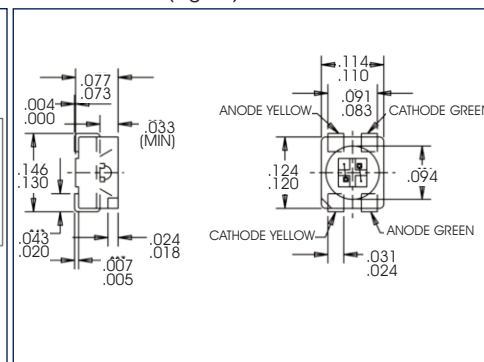
PLCC-4 Bi-Color (Fig 26)
