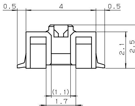
SECT. E-E
