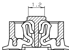
SECT. E-E
