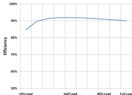
Fig. 5: 12Vin Combined Efficiency, 5V & 3V3 @ 5A, 1V8 & 1V @ 8A, 5V & 3V3 - FET: FDS8984; Inductor: 744314490 7x7x5mm 1V8 & 1V - FETs: Si4946 upper, Si4946 lower; Inductor: 7443551130 13x13x6.5mm
