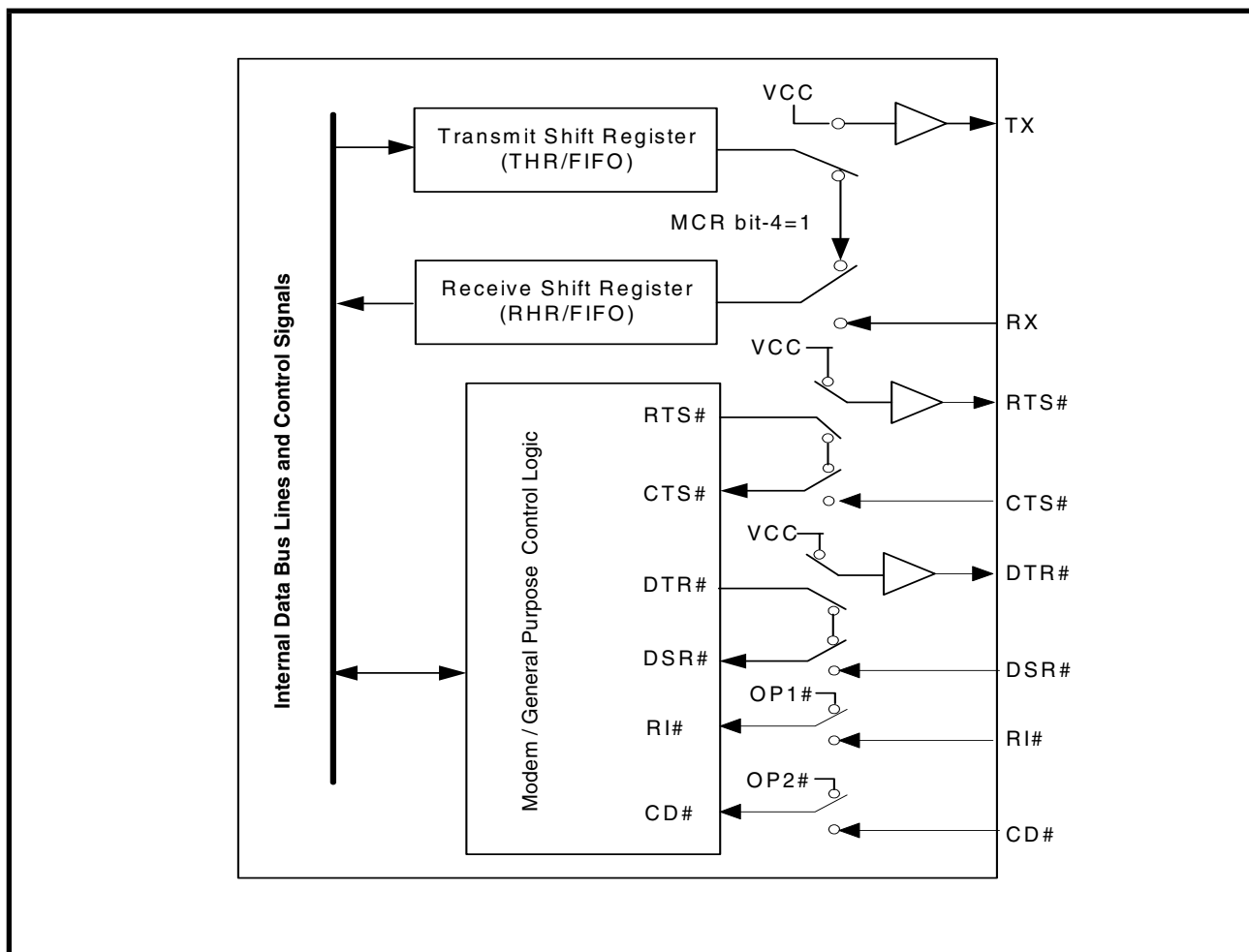
FIGURE 8. INTERNAL LOOPBACK
