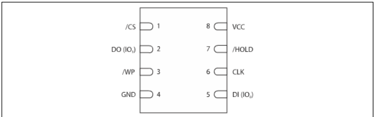
Figure 1b. W25X20CL Pad Assignments, 8-pad WSON 6x5-MM and USON 2x3-MM (Package Code ZP & UX)
