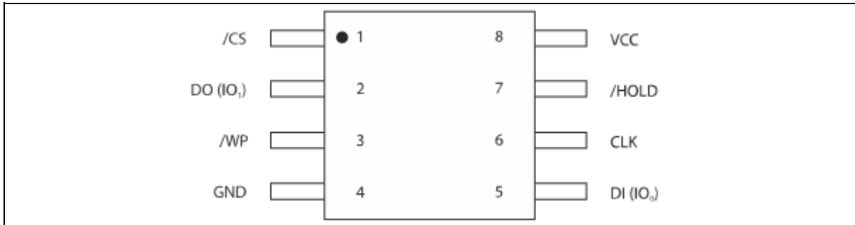
Figure 1a. W25X20CL Pin Assignments, 8-pin SOIC 150-mil, AND VSOP 150-mil (Package Code SN, AND SV)
