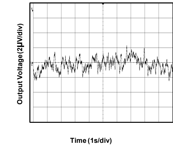
0.1 Hz TO 10 Hz Input Voltage Noise
