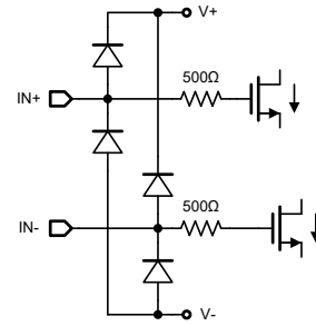
INPUT ESD DIODE CURRENT LIMITING- UNITY GAIN
