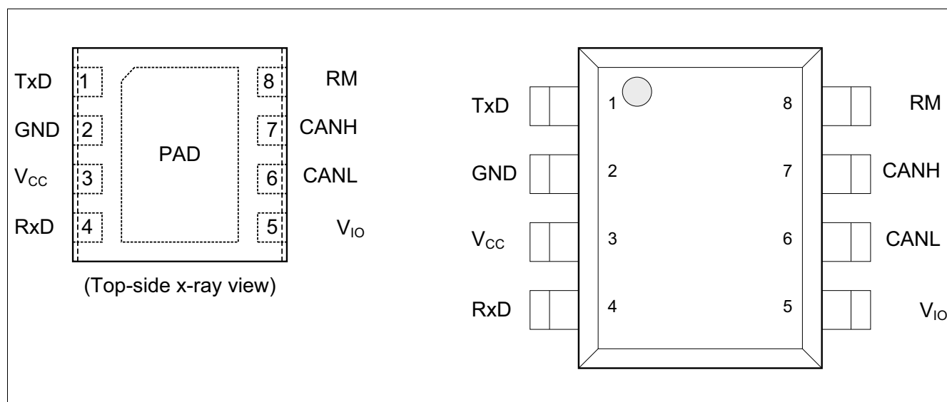
Figure 2 Pin configuration
