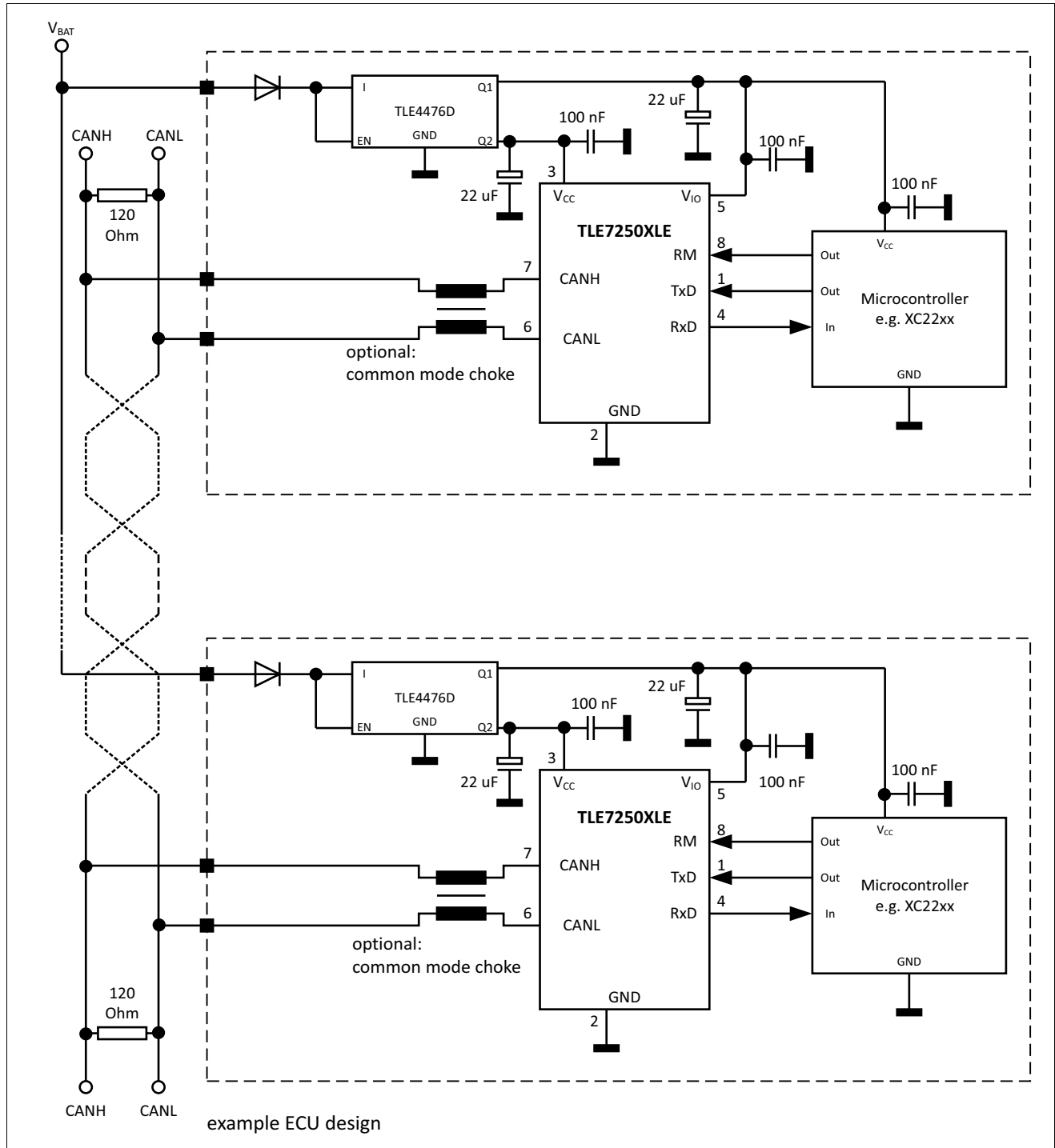
Figure 13 Application circuit
