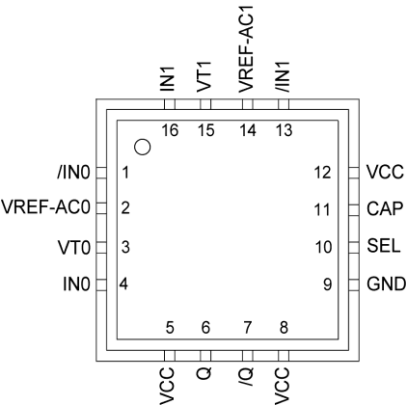
16-Pin QFN (QFN-16)
