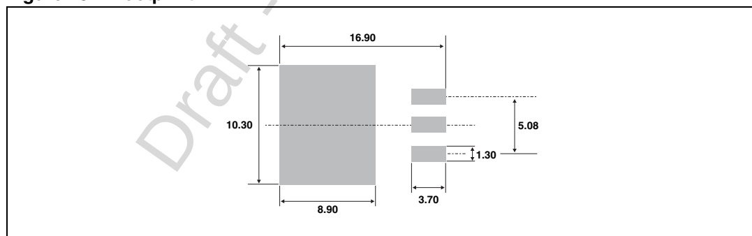
Figure 15. Footprint
