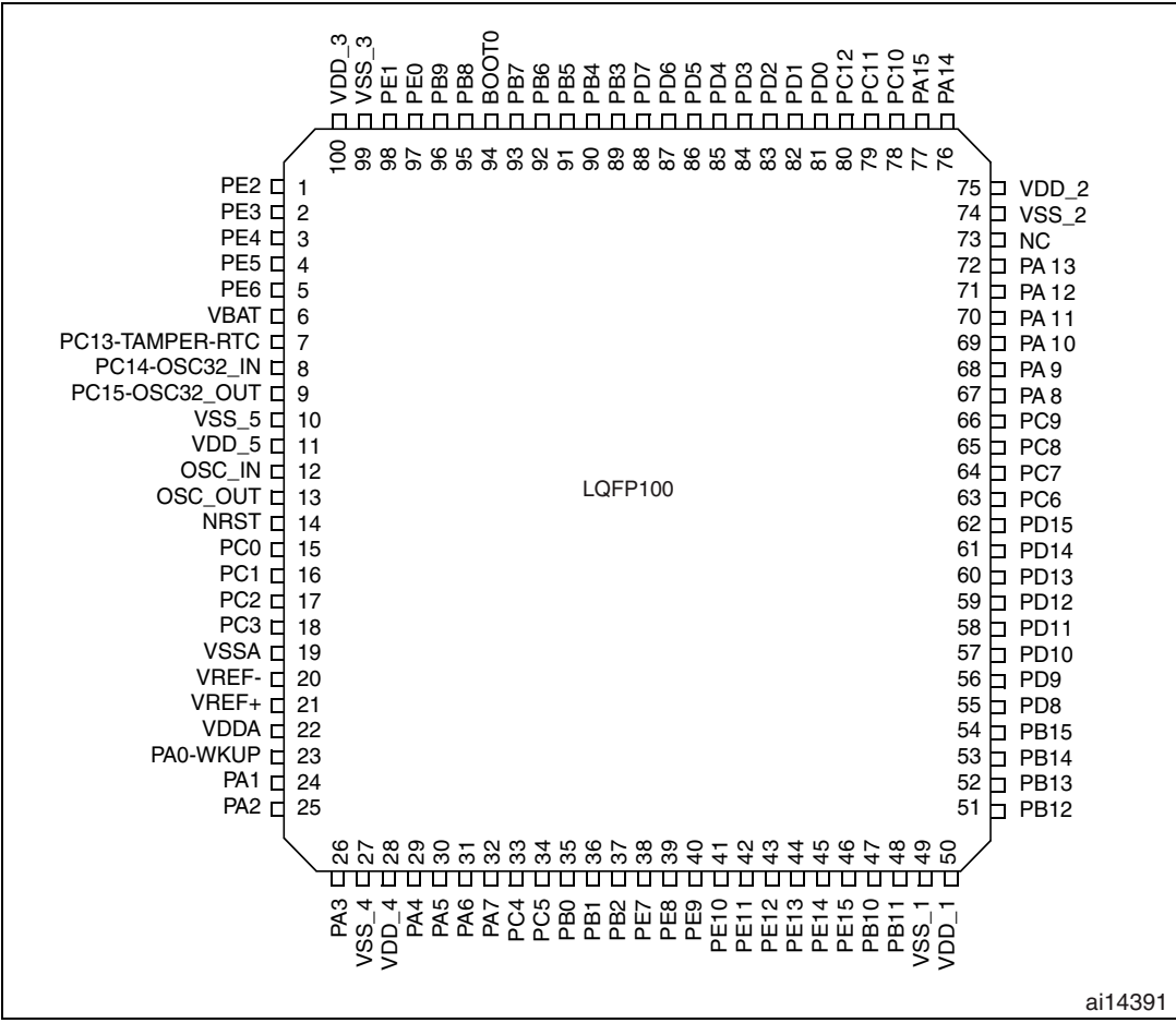
Figure 6. STM32F103xC/D/E performance line LQFP100 pinout
