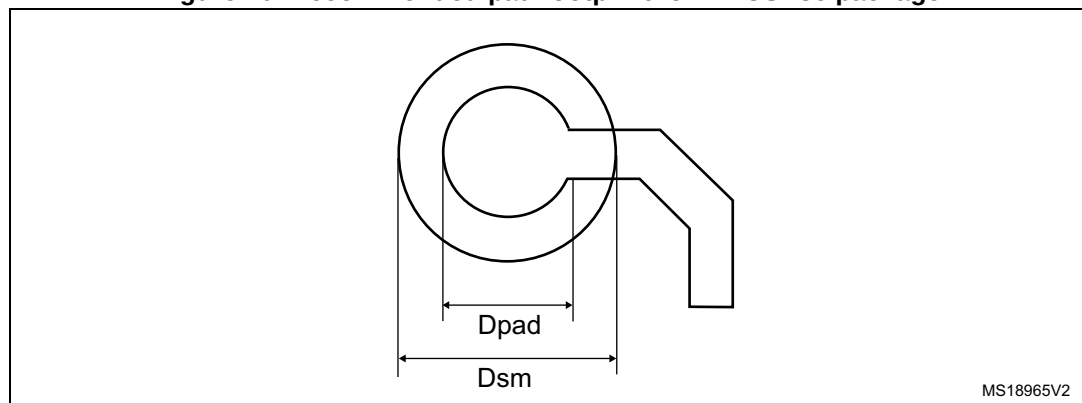
Figure 40. Recommended pad footprint for WLCSP36 package
