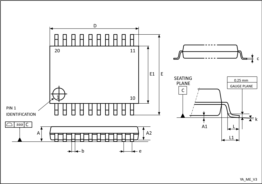
Figure 51.TSSOP20 package outline
