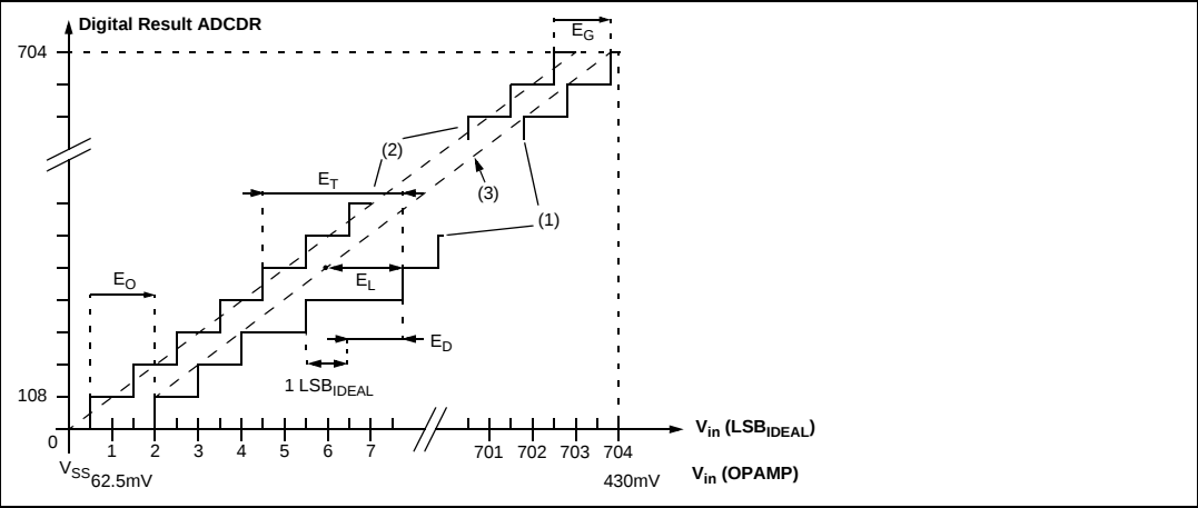
Figure 94. ADC accuracy characteristics with amplifier enabled
