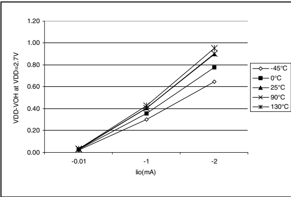
Figure 80. Typical V_{DD}-V_{OH} at V_{DD}=2.7\text{ V}
