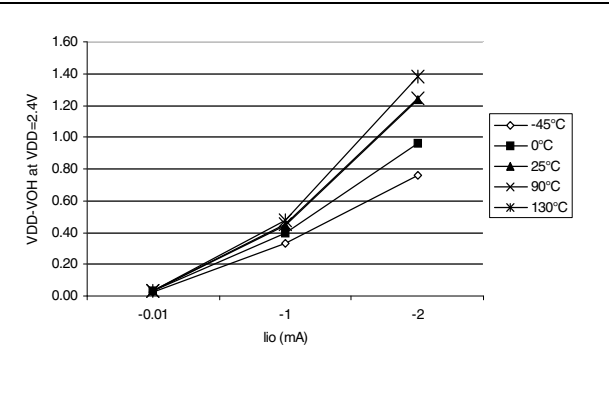
Figure 79. Typical V_{DD}-V_{OH} at V_{DD}=2.4\text{ V}
