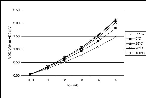
Figure 82. Typical V_{DD}-V_{OH} at V_{DD}=4\text{ V}
