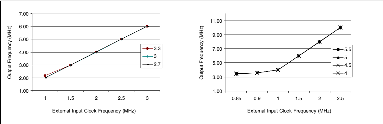
Figure 61. PLLx4 Output vs CLKIN frequency (f OSC = f CLKIN /2*PLL4) Figure 62. PLLx8 Output vs CLKIN frequency (f OSC = f CLKIN /2*PLL8)
