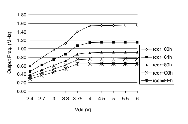
Figure 59. RC Osc Freq vs V_{DD} and RCCR Value
