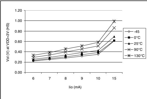
Figure 78. Typical V_{OL} at V_{DD}=3\text{ V} (high-sink)
