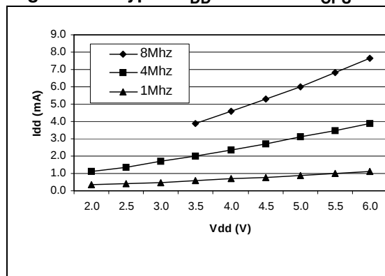
Figure 63. Typical I_{DD} in RUN vs. f_{CPU}
