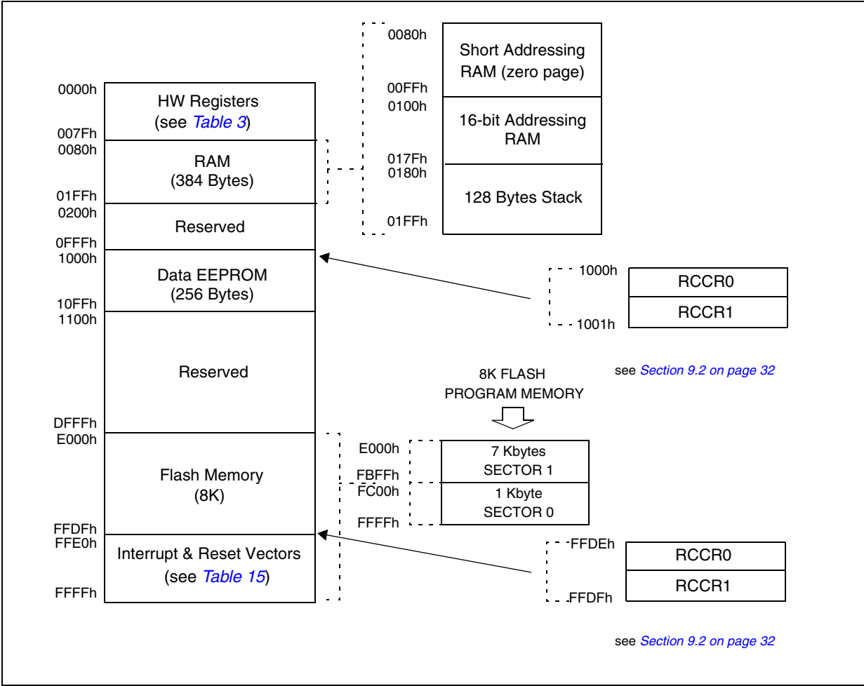
Figure 3. Memory map
