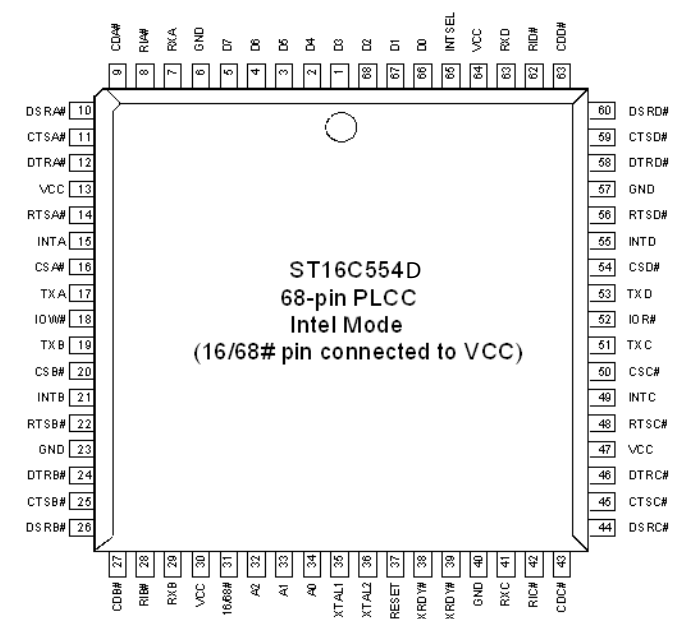
Figure 2: PLCC68 Pinout, Intel Mode
