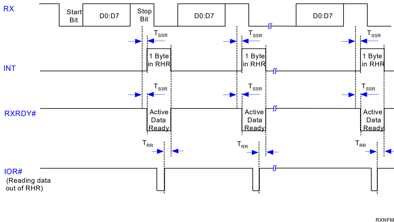
Figure 20: Receive Ready and Interrupt Timing (Non-FIFO Mode) for Channels A - D
