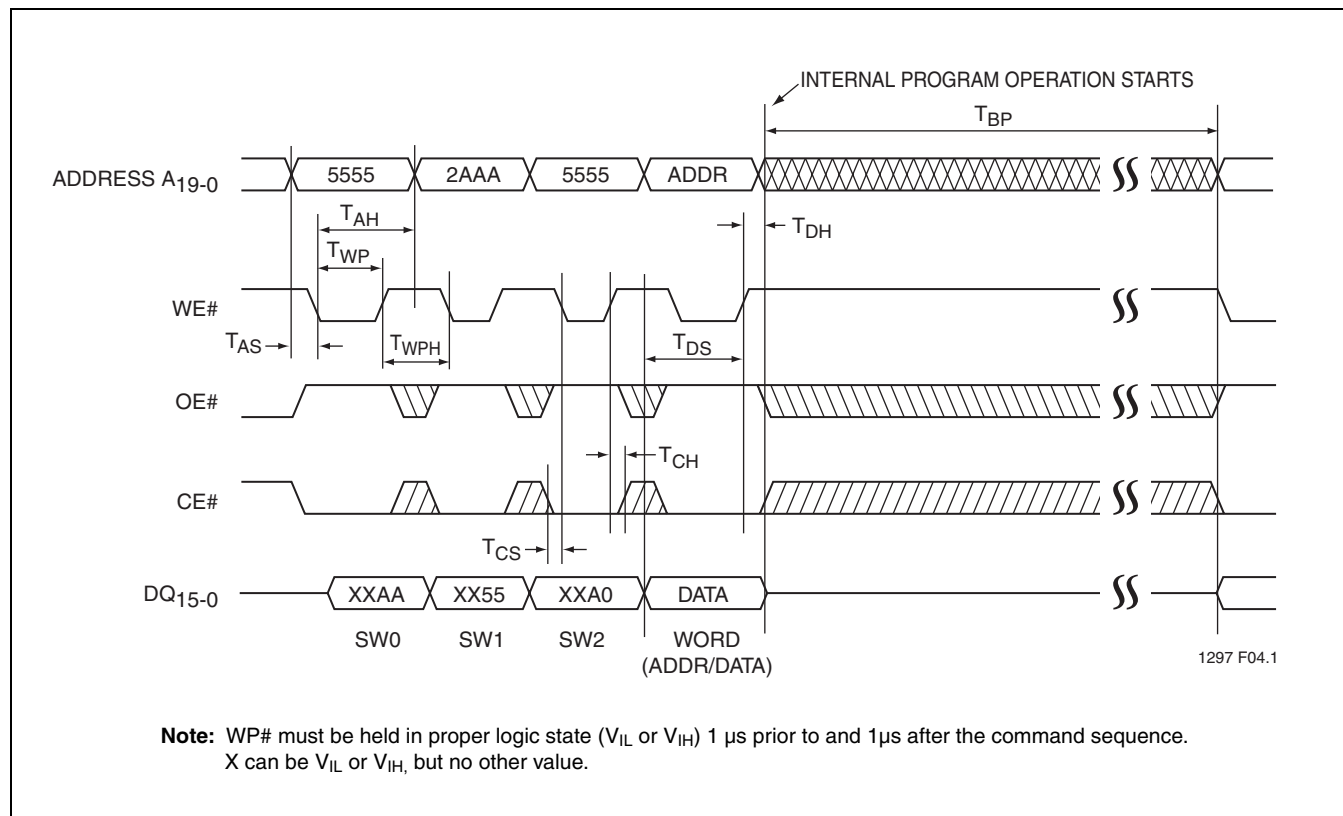
FIGURE 5: WE# Controlled Program Cycle Timing Diagram
