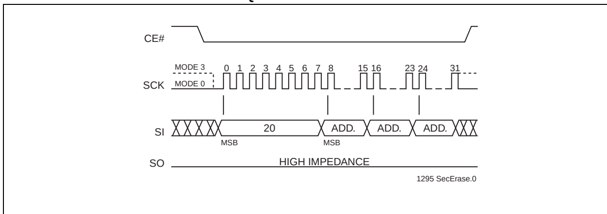
FIGURE 4-10: SECTOR-ERASE SEQUENCE
