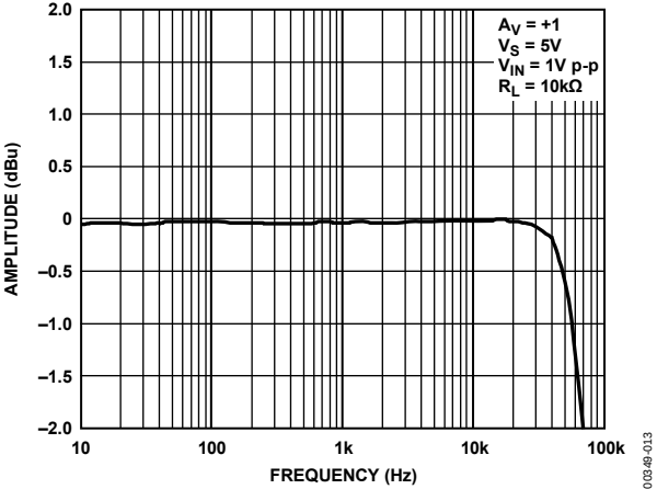
Figure 13. Frequency Response
