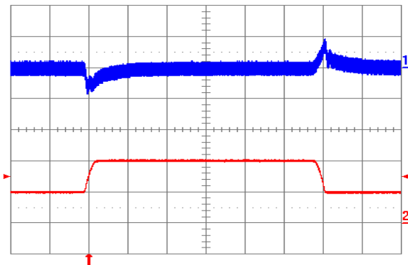
Fig. 2.5V.5: Output voltage response to load current step-change (5A – 10A – 5A) at V_{in} = 48 V. Top trace: output voltage (100 mV/div.). Bottom trace: load current (5 A/div.). Current slew rate: 0.1 A/ \mu s. C_o = 1 \mu F ceramic. Time scale: 0.2 ms/div.
