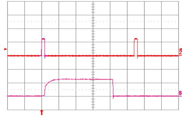
Fig. 1.2V.16: Load current (top trace, 20 A/div., 50 ms/div.) into a 10 mΩ short circuit during restart, at Vin = 48 V. Bottom trace (20 A/div., 5 ms/div.) is an expansion of the on-time portion of the top trace.
