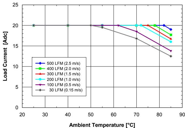
Fig. 1.2V.1: Available load current vs. ambient air temperature and airflow rates for SQM48T/S20012 converter with D height pins mounted vertically with air flowing from pin 3 to pin 1, MOSFET temperature \leq 120^\circ\text{C} , V_{in} = 48\text{ V} .
