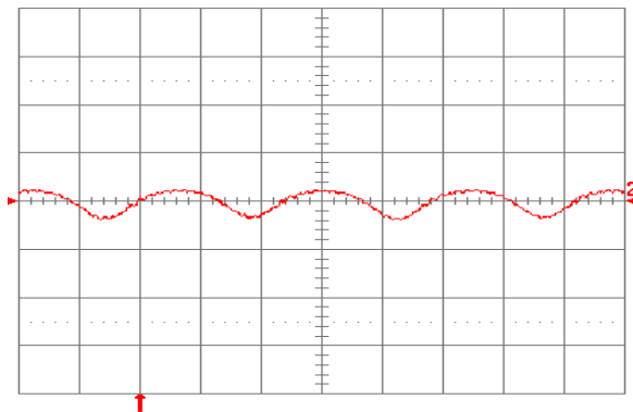
Fig. 1.2V.9: Input reflected ripple current, i_c (100mA/div.), measured at input terminals at full rated load current and V_{in} = 48\ \text{V} . Refer to Fig. 1.2V.8 for test setup. Time scale: 1 \mu\text{s}/\text{div} .
