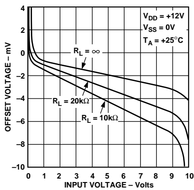
Offset Voltage vs. Input Voltage
