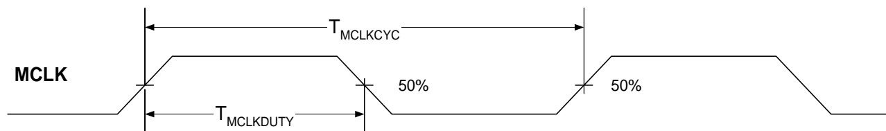
Figure 4.10. MCLK Timings
