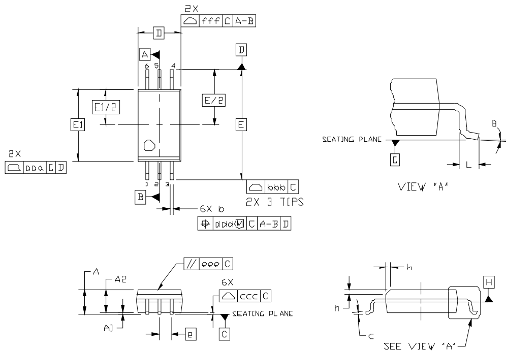
Figure 20. SDIP6 Package
