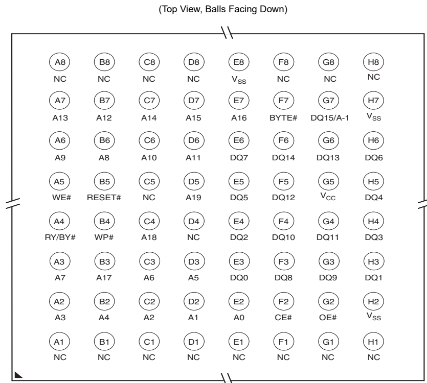
Figure 3. 64-ball Fortified BGA
