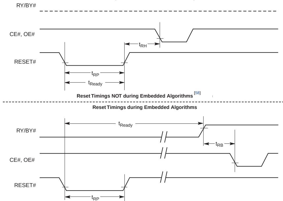
Figure 16. RESET# Timings
