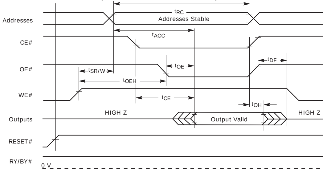
Figure 15. Read Operations Timings
