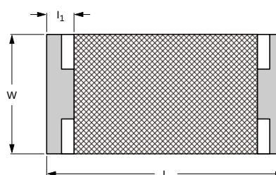
Fig. 5 Chip resistor outlines
