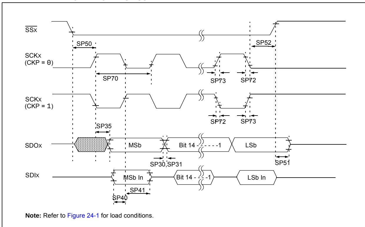
FIGURE 24-16: SPIx SLAVE MODE (FULL-DUPLEX, CKE = 0, CKP = 0, SMP = 0) TIMING CHARACTERISTICS
