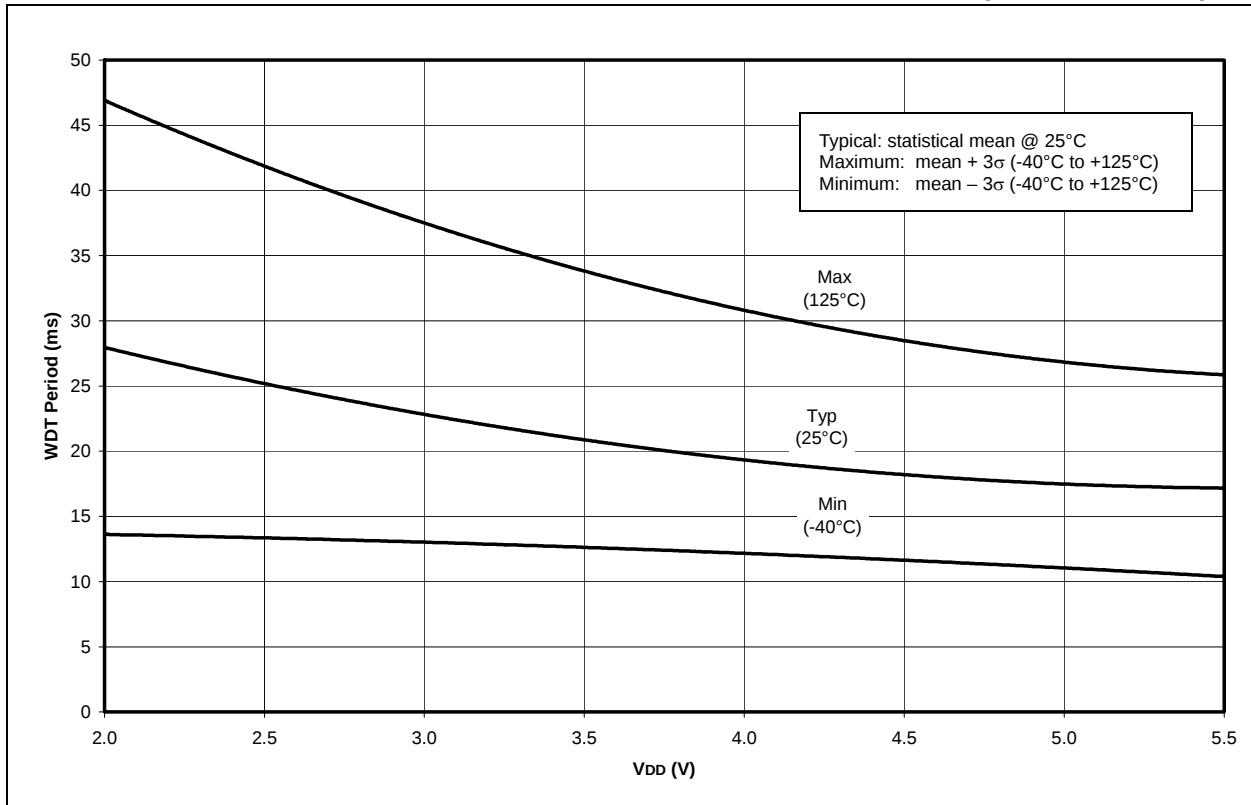
FIGURE 18-14: TYPICAL, MINIMUM AND MAXIMUM WDT PERIOD vs. V_{DD} ( -40^{\circ}C TO +125^{\circ}C )
