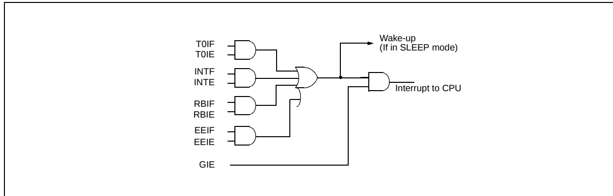
FIGURE 8-16: INTERRUPT LOGIC
