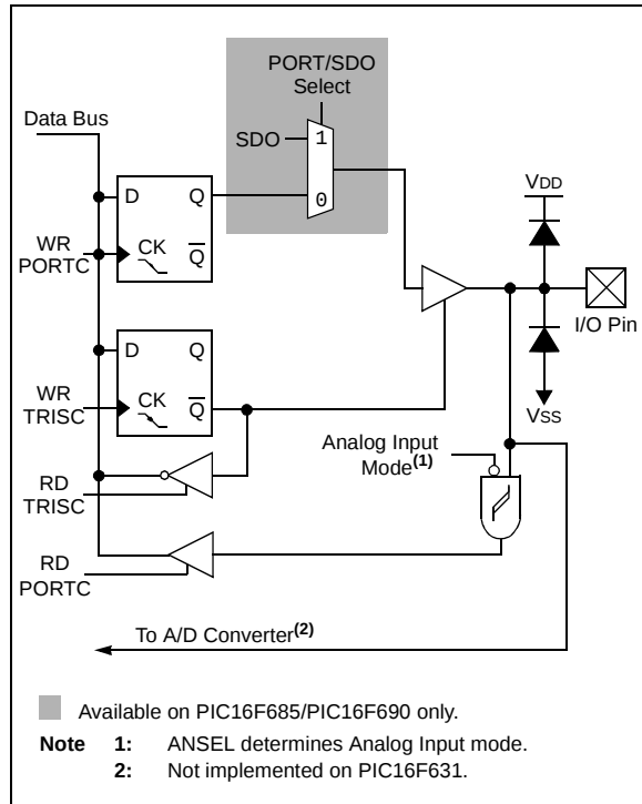
FIGURE 4-16: BLOCK DIAGRAM OF RC7
