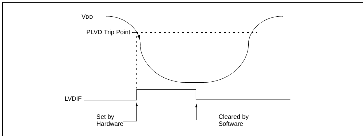
FIGURE 8-2: PLVD OPERATION
