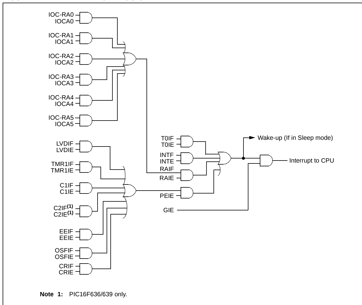
FIGURE 12-7: INTERRUPT LOGIC
