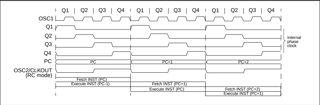
FIGURE 3-4: CLOCK/INSTRUCTION CYCLE
