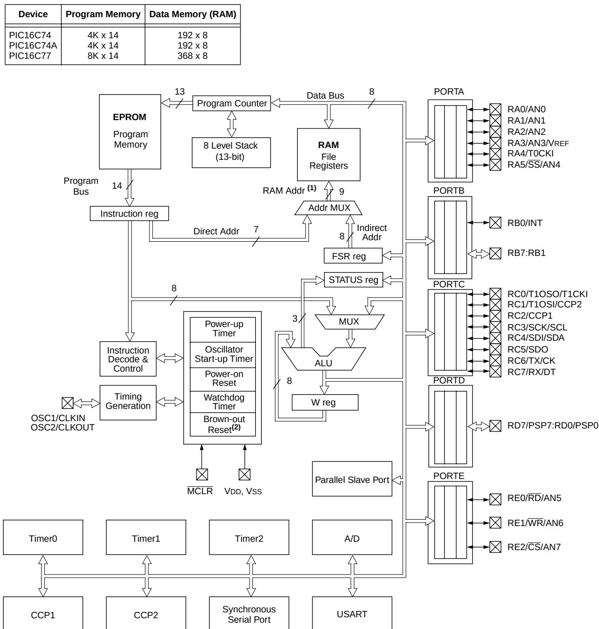
FIGURE 3-3: PIC16C74/74A/77 BLOCK DIAGRAM
