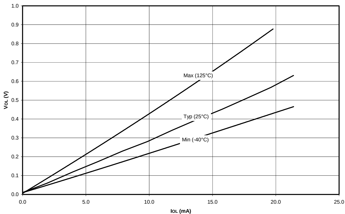
FIGURE 16-29: V_{OH} VS. I_{OH} ( -40^{\circ}\text{C} TO +125^{\circ}\text{C} , V_{DD} = 3.0\text{V} )
