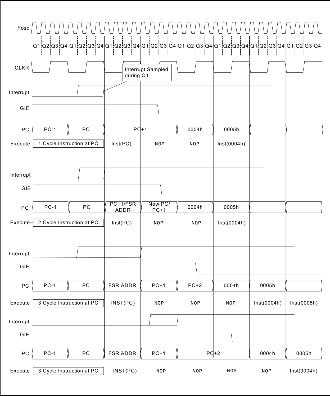
FIGURE 7-2: INTERRUPT LATENCY
