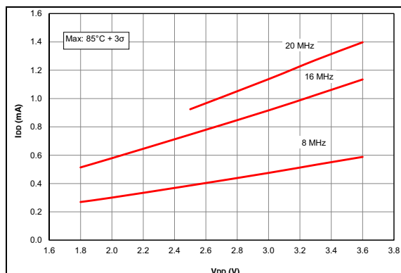
FIGURE 22-6: I_{DD} , Maximum, EC Oscillator, High-Power Mode
