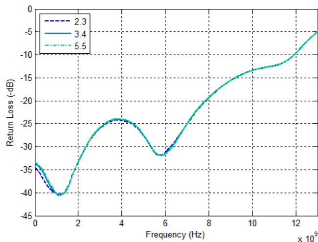
Figure 19. Terminated Port Return Loss vs. V_{DD} (RF1 Active)
