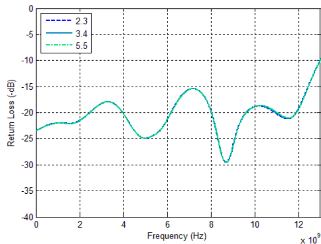
Figure 13. RFC Port Return Loss vs. V_{DD} (RF2 Active)
