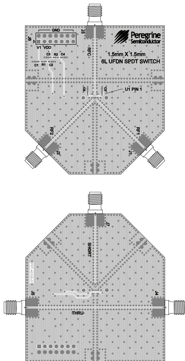
Figure 12 ■ Evaluation Kit Layout for PE42424
