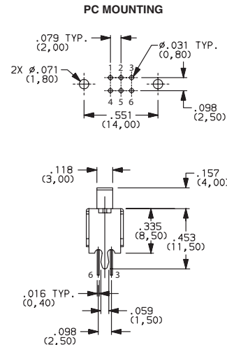
OS202011MV4QN1 DPDT
