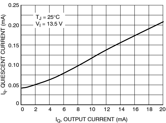
Figure 19. Quiescent Current vs. Output Current (Low Load)
