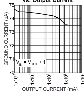
Ground Current vs. Output Current
