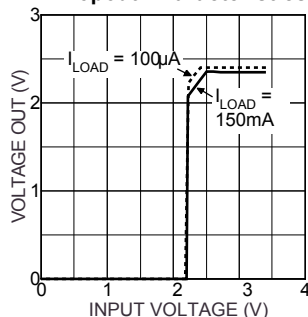
Dropout Characteristics
