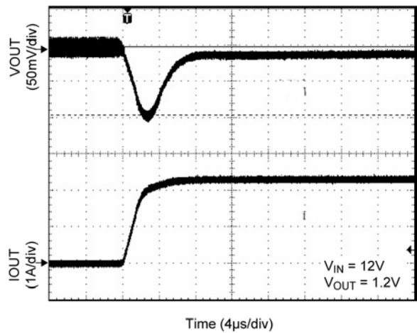
Transient Response
